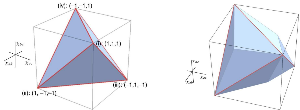
Figure 3. At the left: the tetrahedron of triplets of anti-correlation coefficients (\chi_{ab}, \chi_{ac}, \chi_{bc}) allowed by local hidden-variable theories in the Mermin-style setup (see the end of Section 2 above) for two possible values per balanced random variable. At the right: the polyhedron corresponding to the case of three possible values. Note that whenever there are more than two values per variable, the corresponding correlation polytope will have more than three dimensions. The three-dimensional polyhedron at the right is obtained by considering only the hidden-variable theories that are admissible in the sense of having uniform marginals for the probabilities of Alice’s and Bob’s experimental outcomes, respectively, and obey certain other symmetry conditions which are necessary in order to simulate the corresponding quantum correlations [49, ch. 4]. Source: [49, pp. 40, 140].
